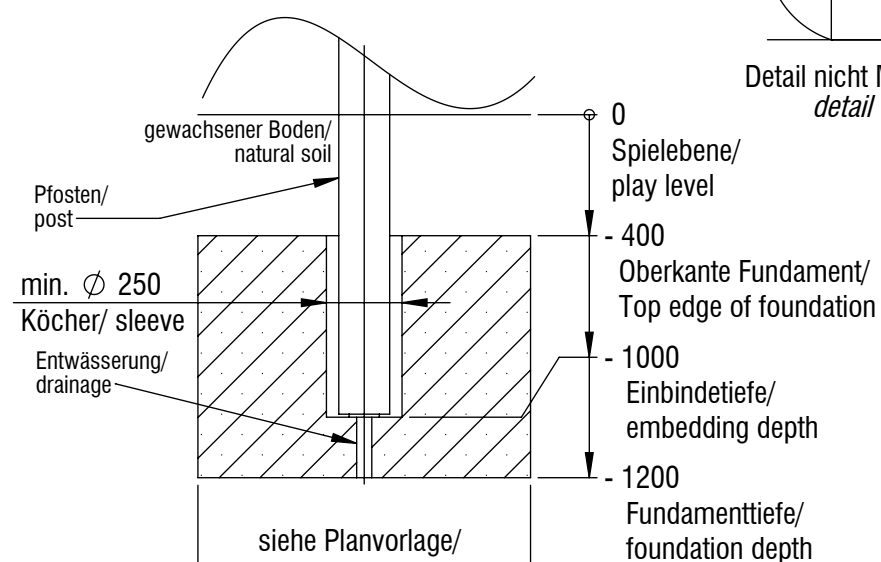
Fundamentschnitt Pfosten / foundation cut section post SP01
