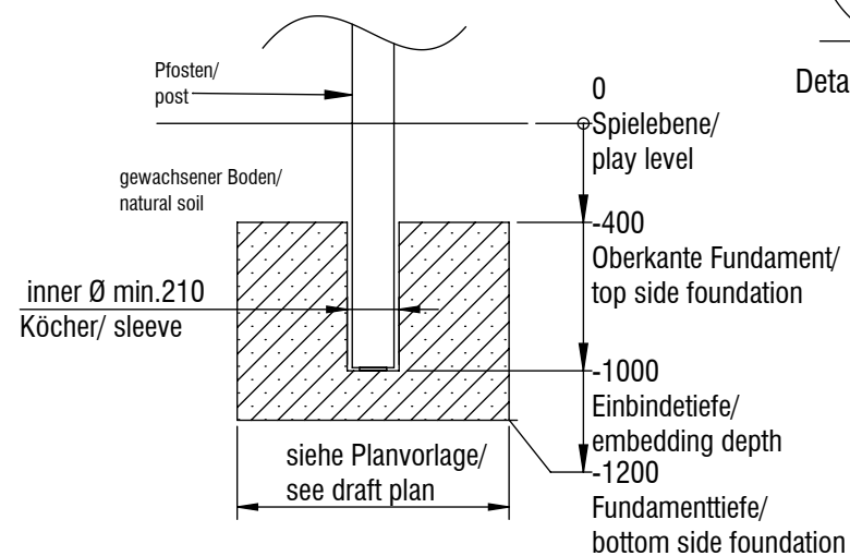
Fundamentschnitt Pfosten / foundation cut section post SP01
