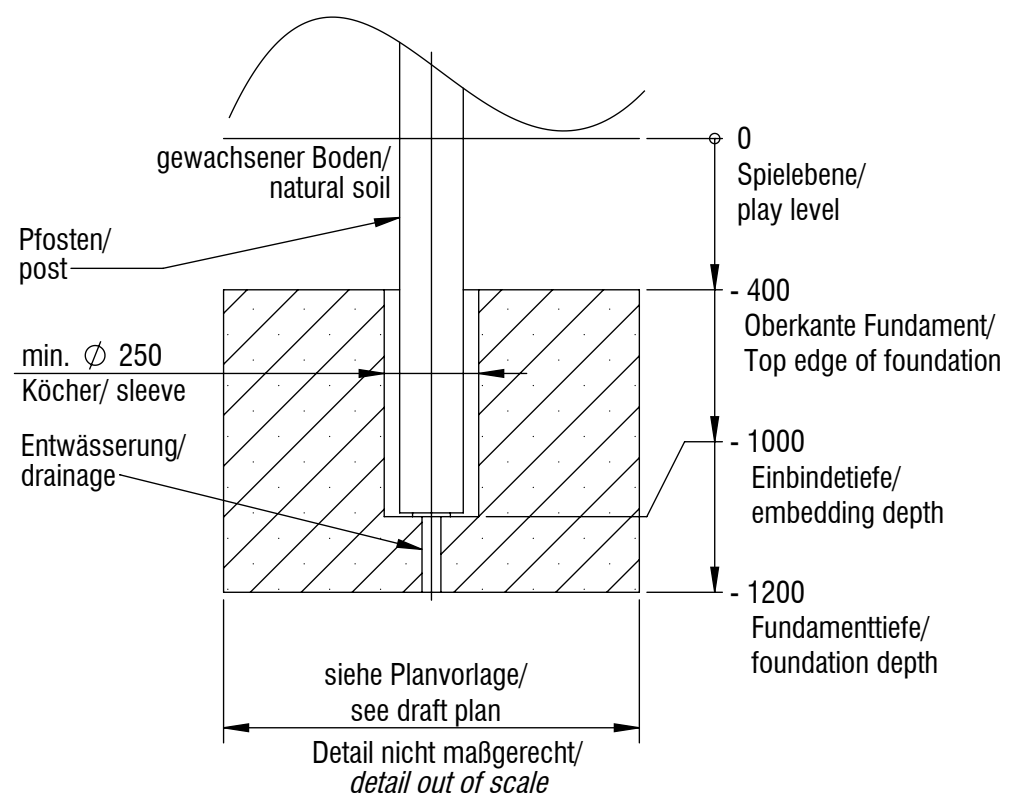
Fundamentschnitt Pfosten / foundation cut section post SP01
