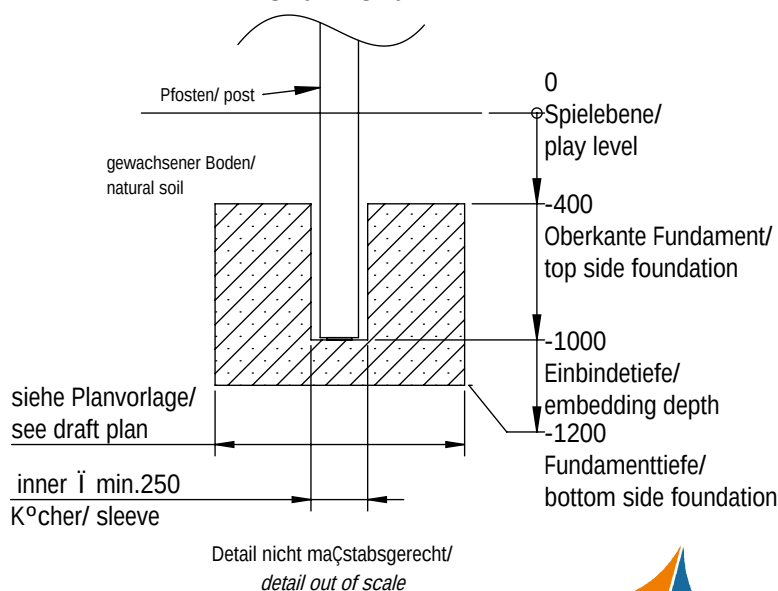
Fundamentschnitt Pfosten/ foundation cut section post SP01 - SP04
