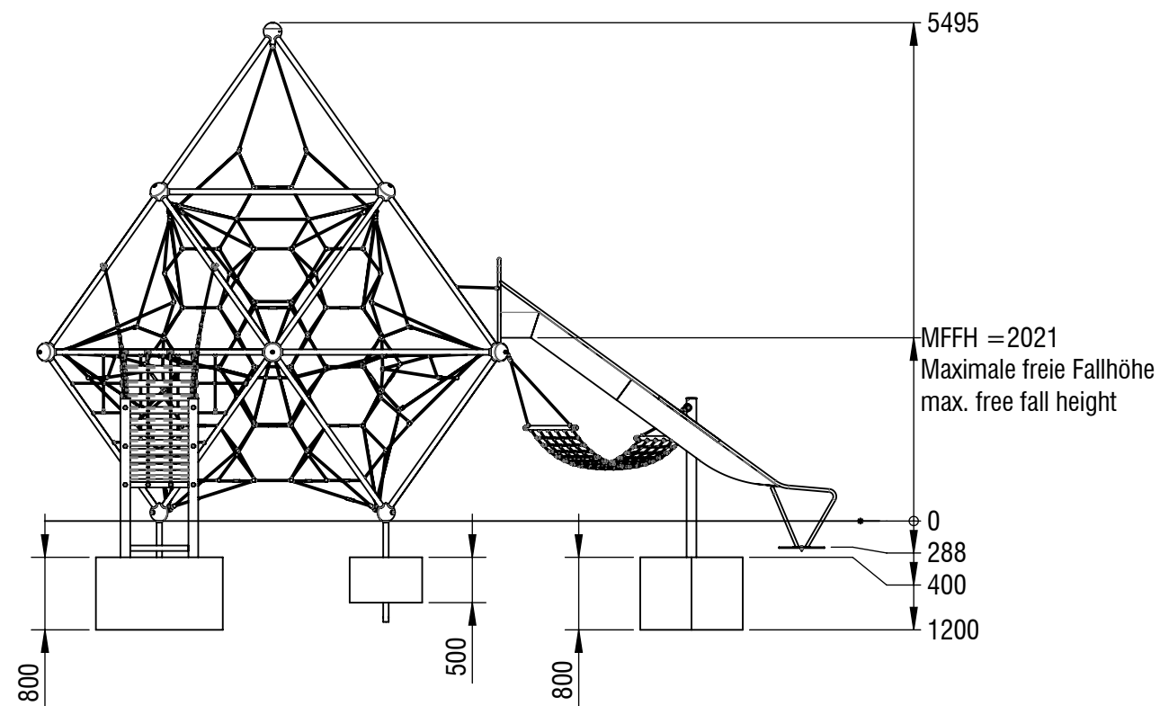
Fundamentanker/ Foundation anchor
