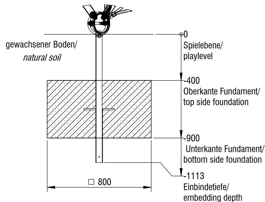
Fundamentanker/ Foundation anchor
