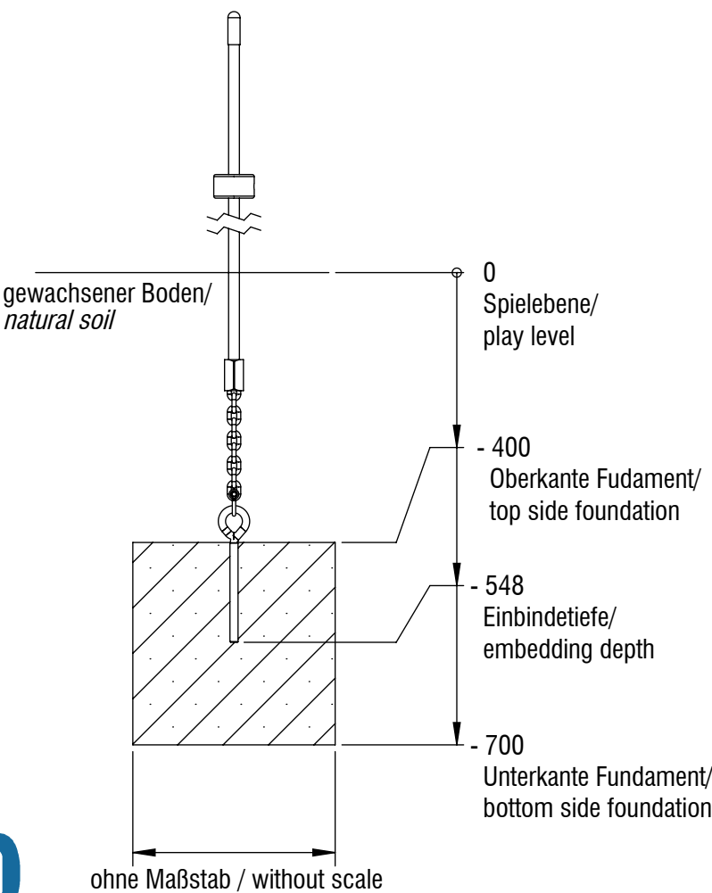
Fundamentschnitt Kletterseil/ foundation cut climbing rope
