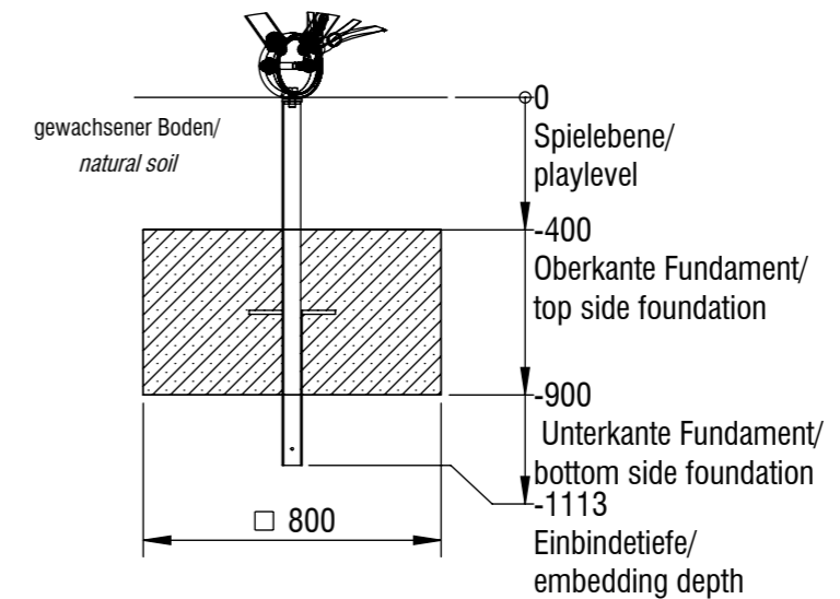
Fundamentalschnitt / foundation cut Fundamentanker / foundation anchor
