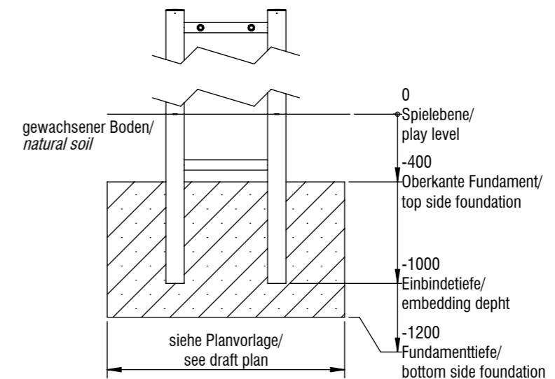
Fundamentalschnitt H-Stütze / foundation cut H-post HS01, HS02, HS03
