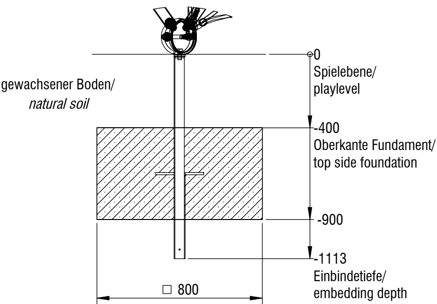
Fundamentanker concrete anchor foundation
