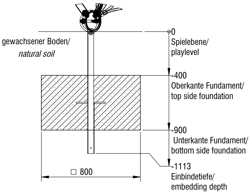
Fundamentanker concrete anchor foundation
