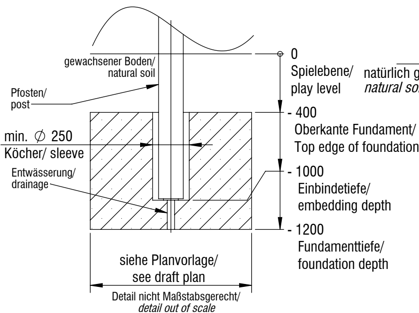
Fundamentschnitt Pfosten SP01 / foundation cut post SP01
