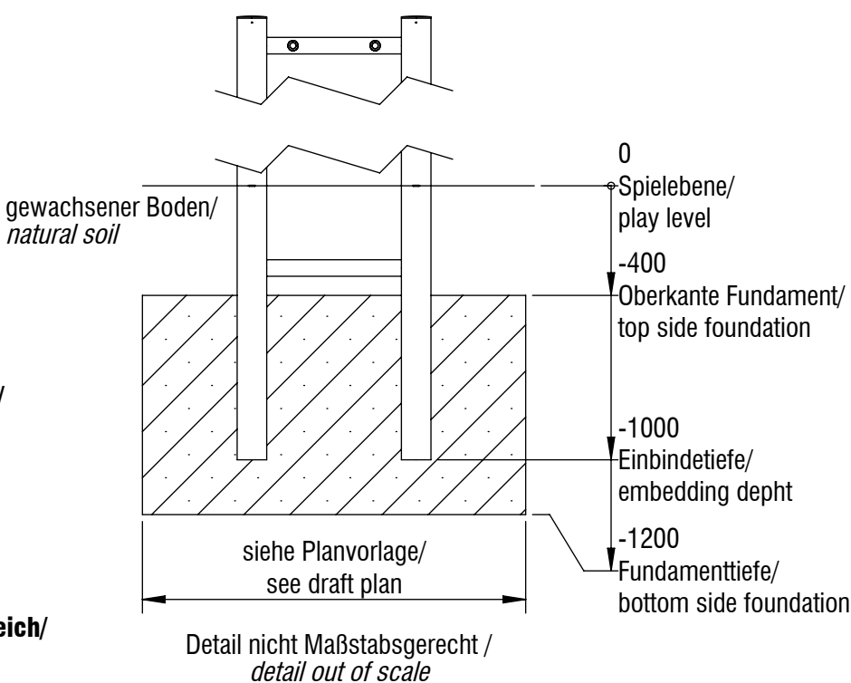
Fundamentschnitt Pfosten SP01 / foundation cut post SP01
