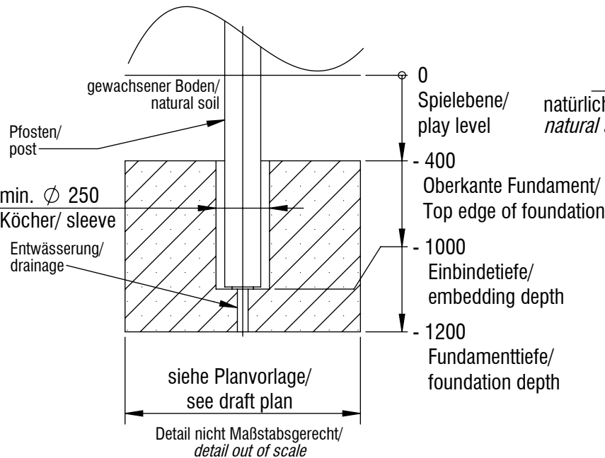
Fundamentschnitt Pfosten SP01 / foundation cut post SP01
