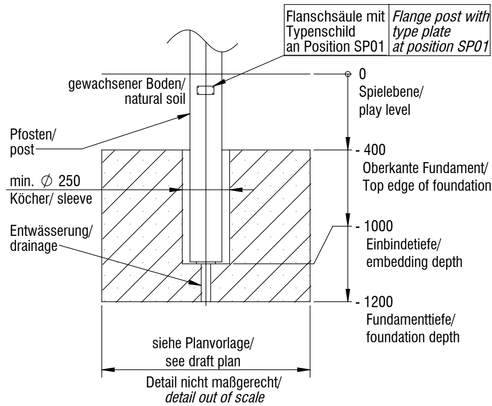
Fundamentschnitt Adventure Park Pfosten / foundation cross section for Adventure Park posts SP01-SP10
