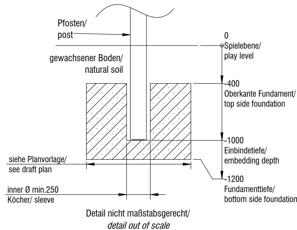
Fundamentschnitt Adventure Park Pfosten / foundation cross section for Adventure Park posts SP01-SP10
