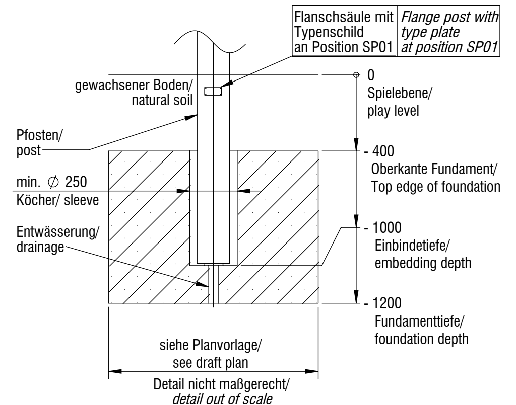
Fundamentschnitt Pfosten / foundation cut posts SP01-SP06
