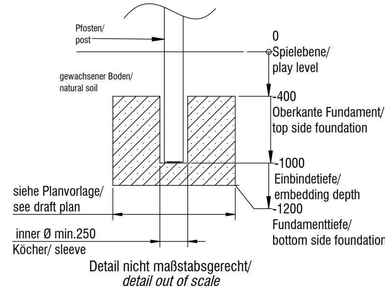
Fundamentschnitt Pfosten / foundation cut posts SP01-SP06
