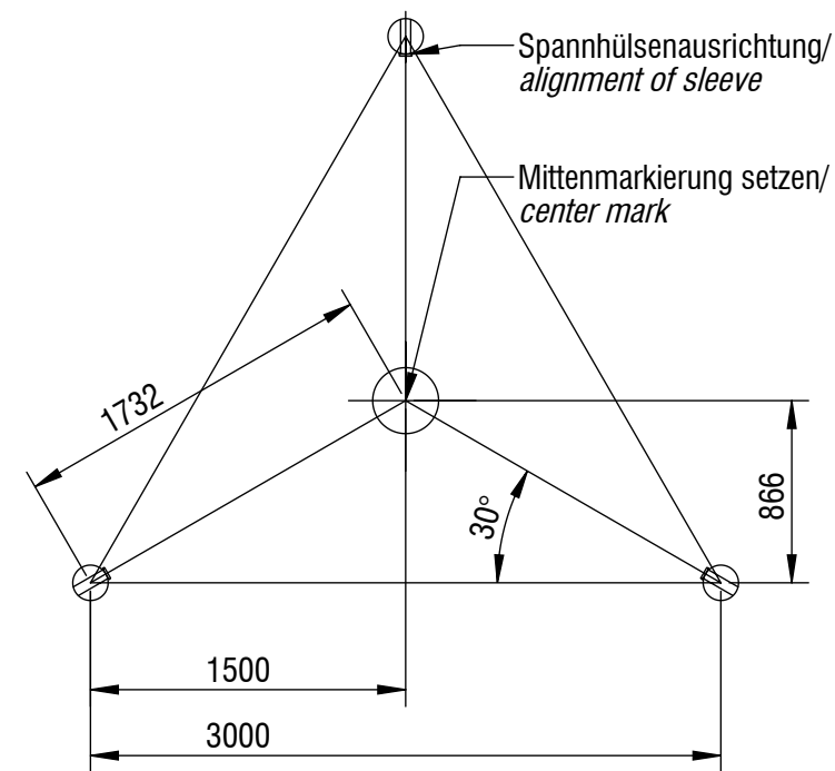
Ausrichtung Adventure Park / alignment for Adventure Park Spinnennetz / spider web, Orchideenblatt / orchid leaf
