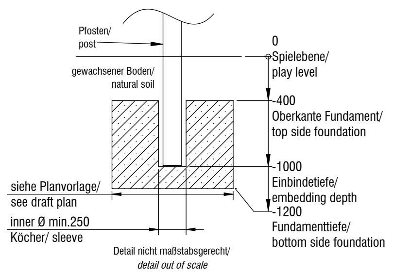
Fundamentschnitt Adventure Park Pfosten / foundation cut adventure park post SP01, SP02, SP03, FS03, FS04, FS05
