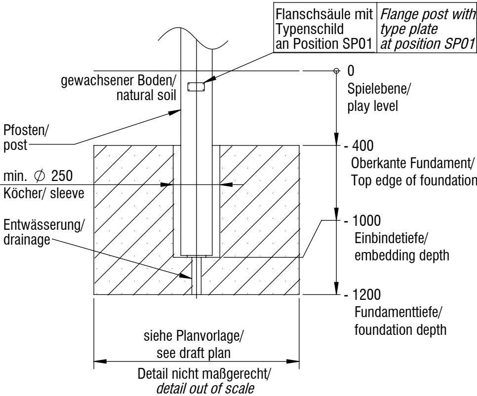
Fundamentschnitt Pfosten / foundation cut posts SP01 - SP04
