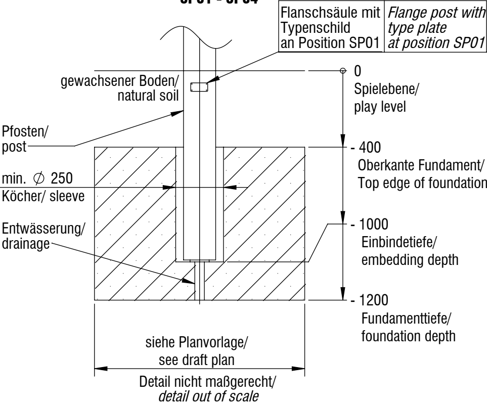
Fundamentschnitt Pfosten/ foundation cut post SP01 - SP04
