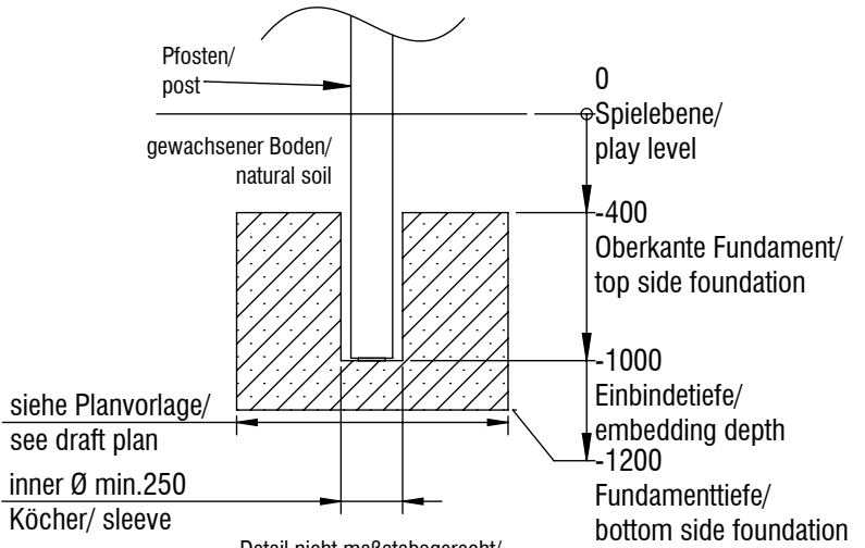
Fundamentschnitt Adventure Park Pfosten / foundation cut adventure park post SP01, SP02, SP03, FS03, FS04, FS05
