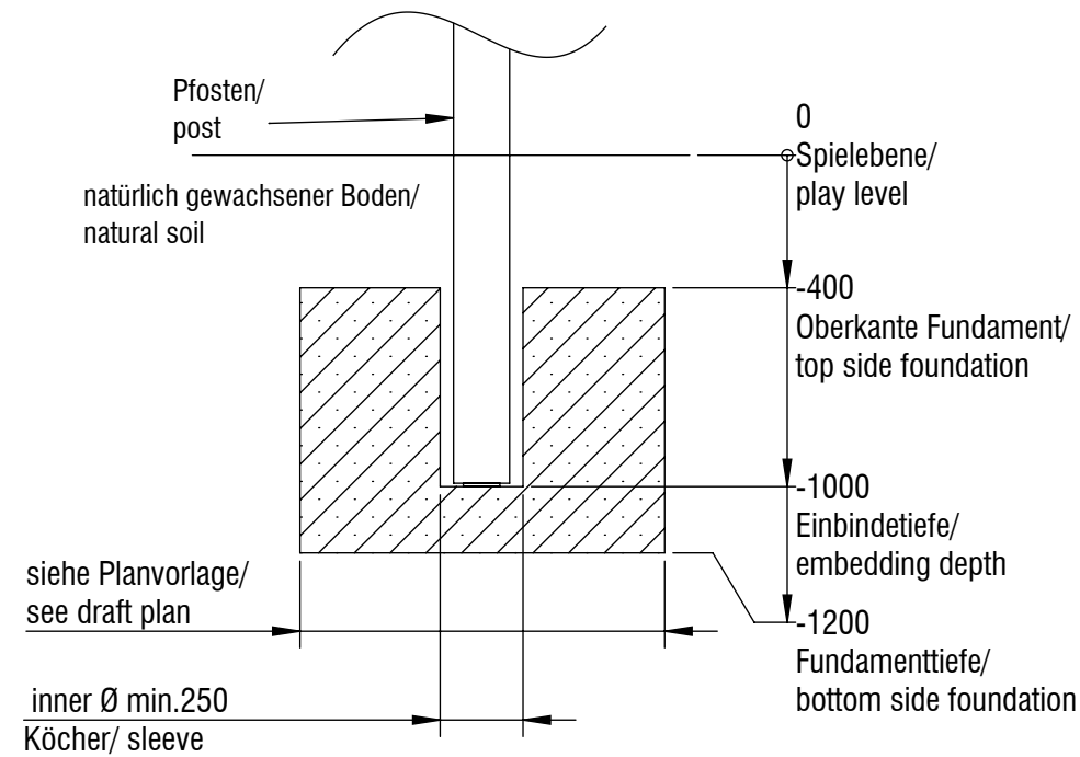
Fundamentschnitt Pfosten/ foundation cut posts SP01 - 04
