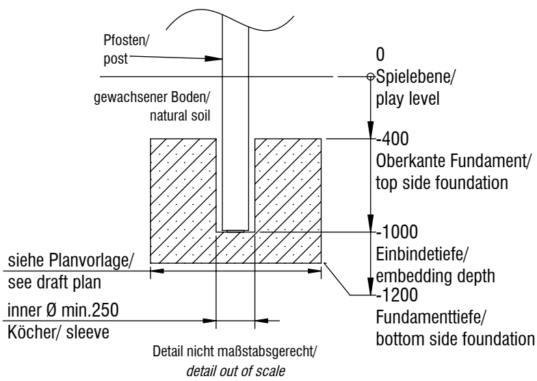
Fundamentschnitt / foundation cut SP01, SP02
