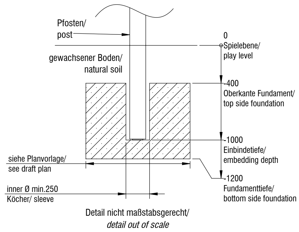
Fundamentschnitt Pfosten/ foundation cut section post SP01 - SP10
