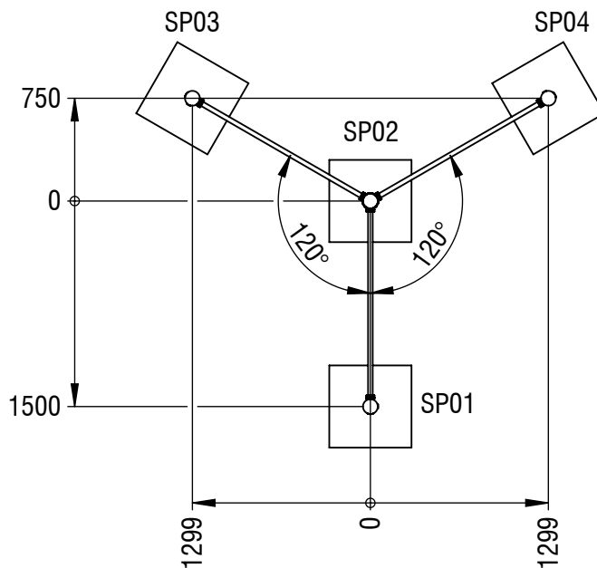
Fundamentalschnitt Pfosten/ foundation cut section post SP01 - SP04
