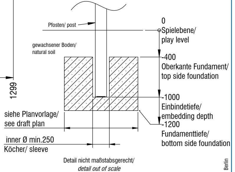
Fundamentalschnitt Pfosten/ foundation cut section post SP01 - SP04
