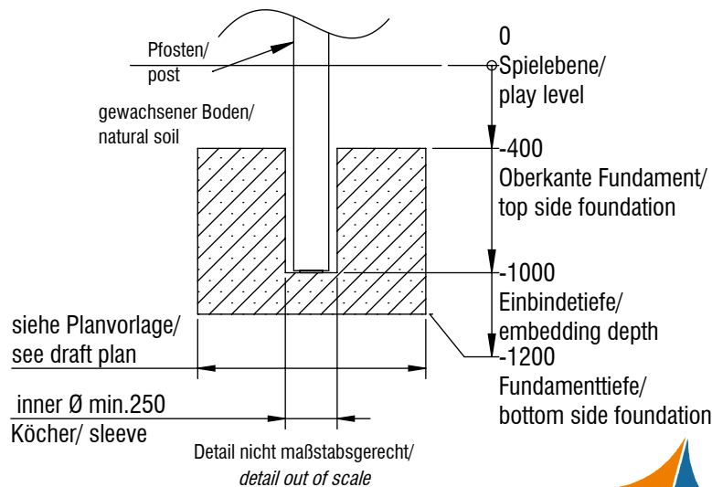
Fundamentschnitt Pfosten/ foundation cut section post SP01 - SP04
