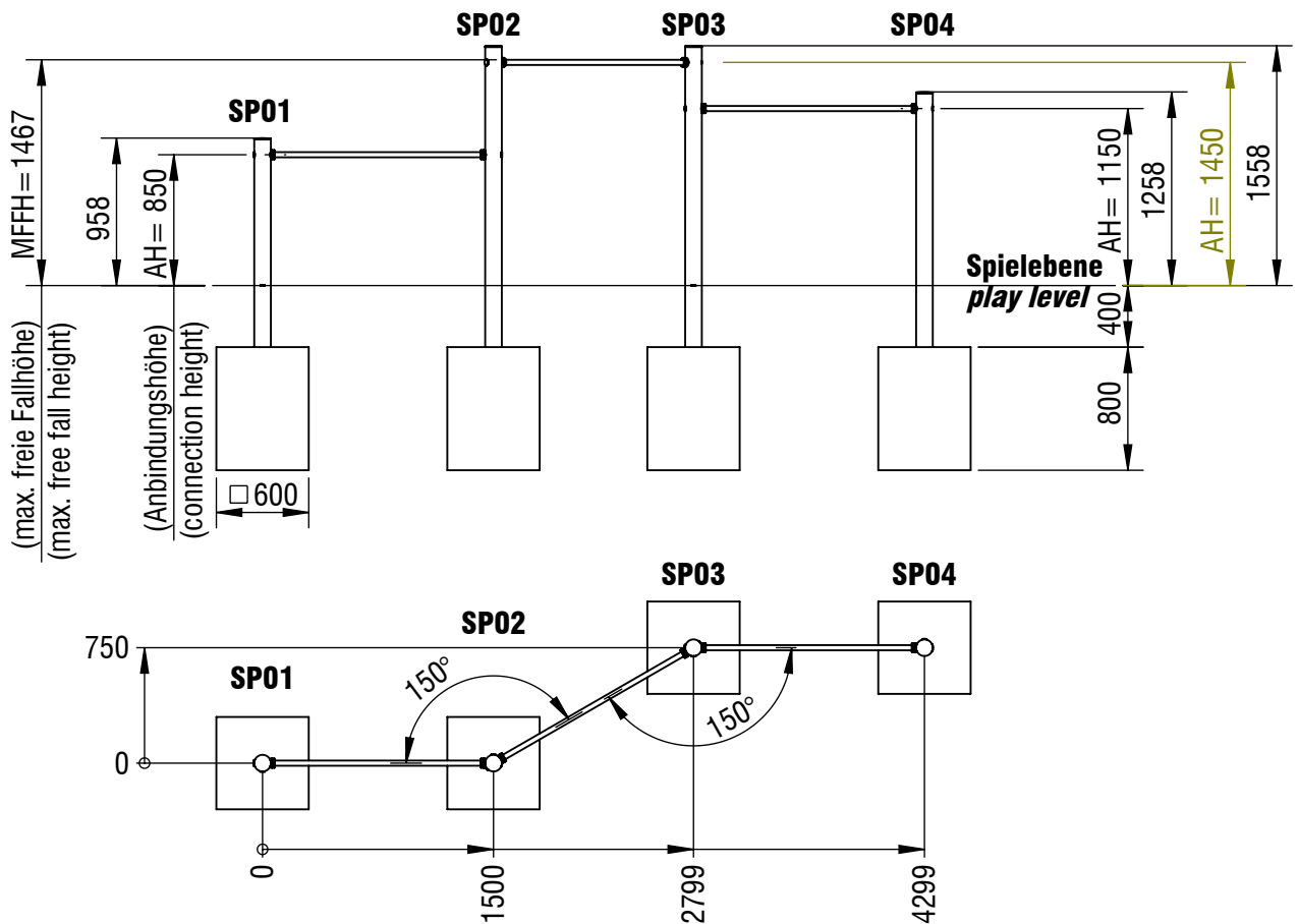
Fundamentschnitt Pfosten/ foundation cut section post SP01 - SP04
