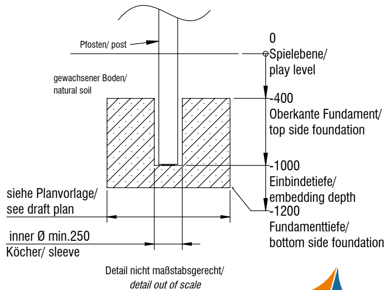
Fundamentschnitt Pfosten/ foundation cut section post SP01 - SP04
