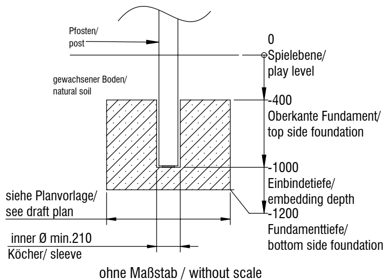
Fundamentschnitt Pfosten/ foundation cut section post SP01 - SP03
