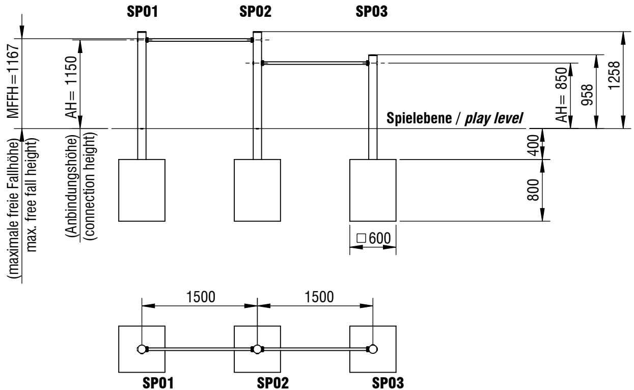
Fundamentschnitt Pfosten/ foundation cut section post SP01 - SP03
