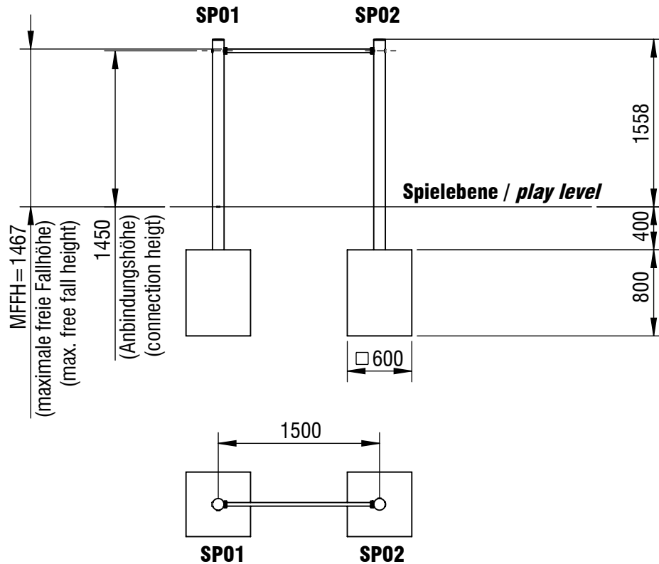
Fundamentschnitt Pfosten/ foundation cut section post SP01 - SP02
