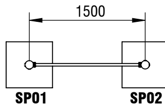
Fundamentschnitt Pfosten/ foundation cut section post SP01 - SP02
