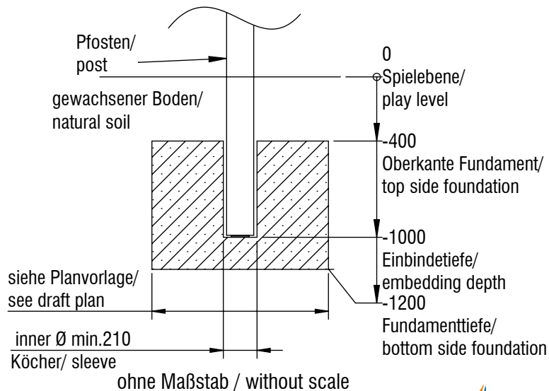
Fundamentschnitt Pfosten/ foundation cut section post SP01 - SP02
